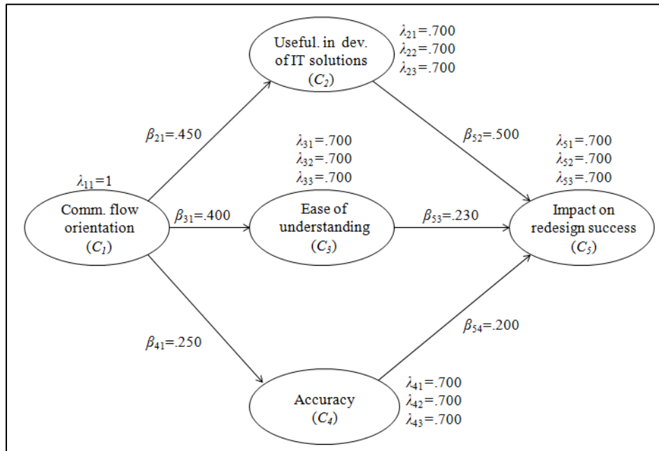
Figure 2. True population model
